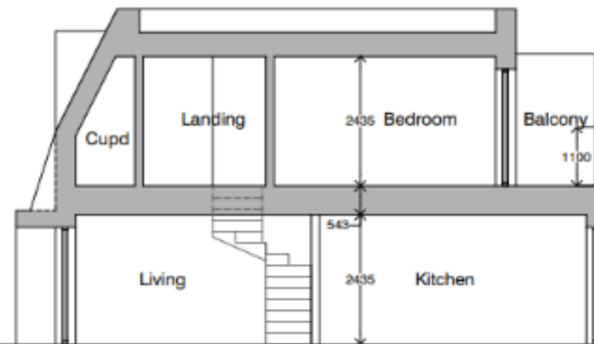
06 PROPOSED SECTION AA 1:100
