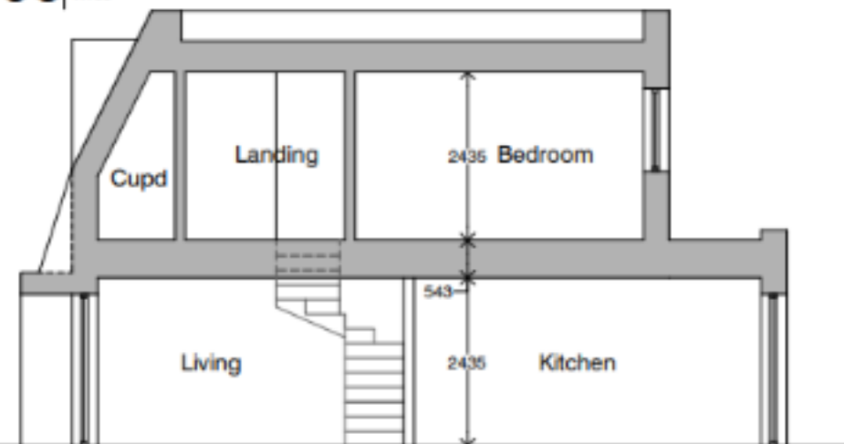
07 PROPOSED SECTION AA (alternative with balcony omitted) 1:100
