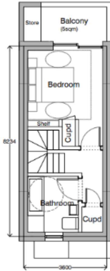
02 PROPOSED FIRST FLOOR PLAN 1:100
