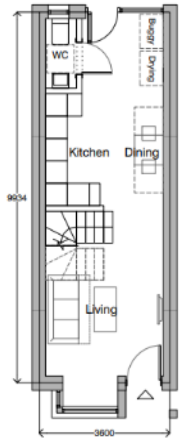
01 PROPOSED GROUND FLOOR PLAN 1:100
