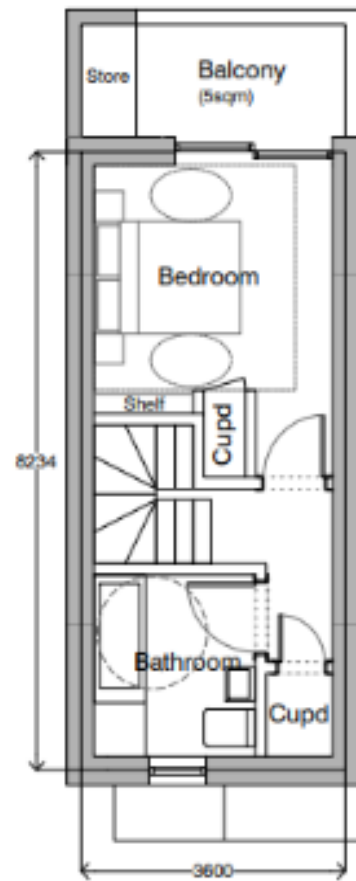
02 PROPOSED FIRST FLOOR PLAN 1:100
