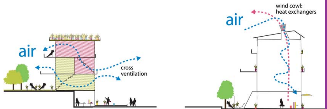
Figure 6 Natural Ventilation
